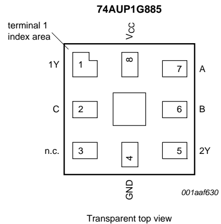
Fig 5. Pin configuration SOT902-2
