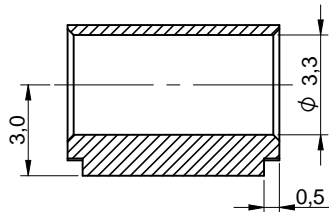
sectional drawing A-A
