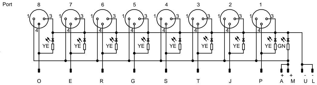
Pin-Configuration M16x0,75
