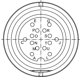
Pin-Configuration M16x0,75
