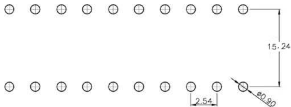
PCB LAYOUT
