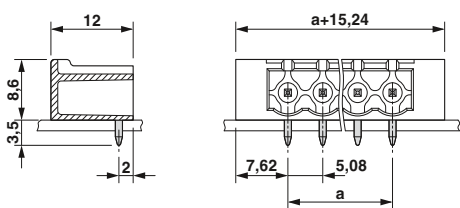
Drilling diagram
