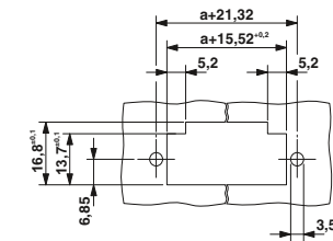
For snap-lock mechanism
