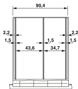
Housing inner dimensions
