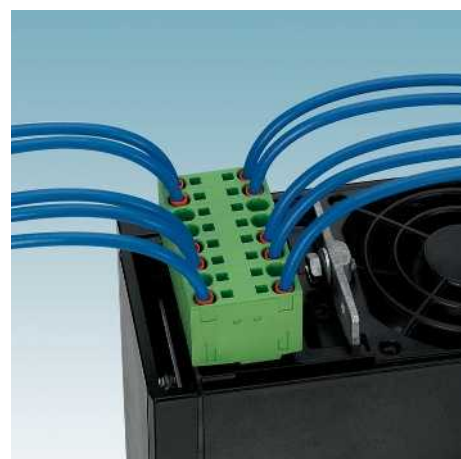
TSPC 5 TWIN plugs with spring connection, 7.62 mm pitch
