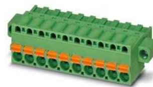
With connection area moved to the top, test connection and screw flange
