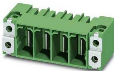
Horizontal, with shield connection, 600 V UL approval
