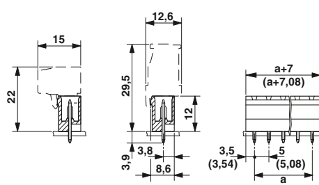
Drilling diagram
