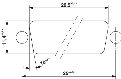
Mounting cutout according to DIN 41652-3 for panel thickness of up to 2.0 mm PSC 1,5/3..M(-PE) See page 251.
