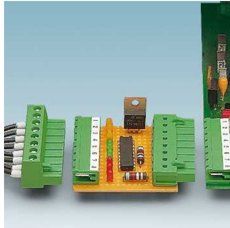
3. IC 2,5 versions and MSTB 2,5 headers to create test, indicator, converter or branch adapters.
