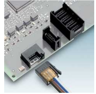
Plug-in connectors with displacement connection and headers with 2.0 mm pitch CIOC...(M)(F) Page 65 CIOC...F(V)(H) Page 67
