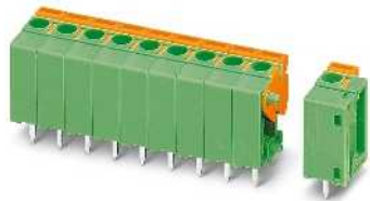
5.08 mm pitch, with opening lever, conductor connection vertical to the PCB
