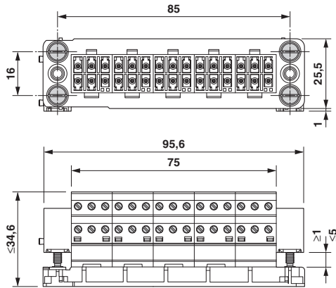
Dimensional drawing
