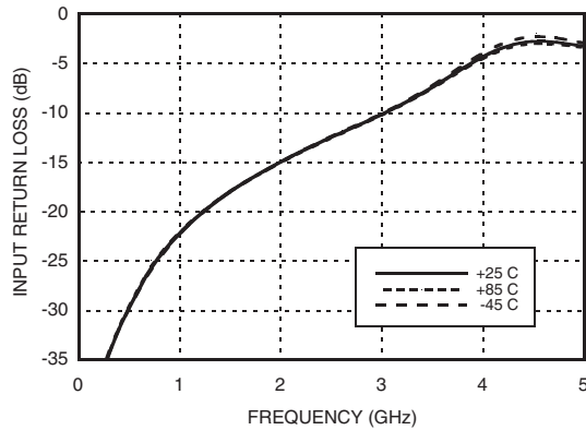
Input Return Loss vs. Frequency, V_{cc} = 3.3V
